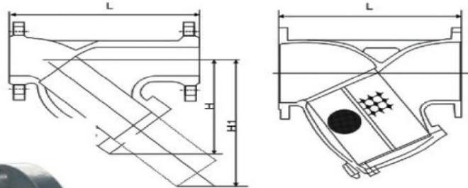
CAST STEEL STAINER CLASS 150
